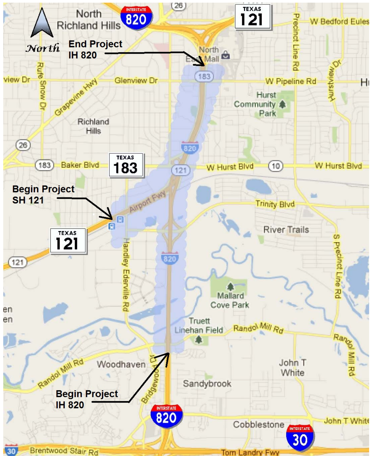
IH 820 Project Location Map From Randol Mill Road to North SH 121 Interchange
